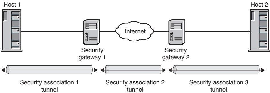
Figure 90. Cascaded tunnels
