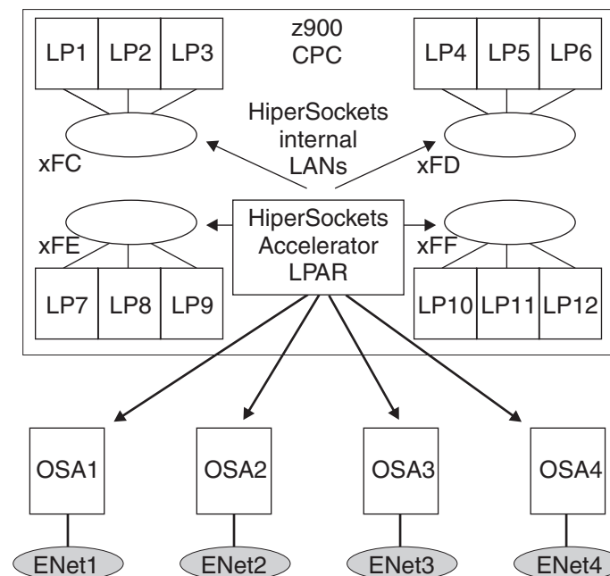
Figure 17. HiperSockets Accelerator configuration
