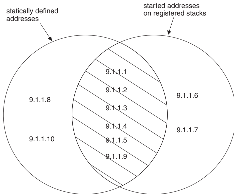
Figure 65. Address association with mvplex.mycorp.com
