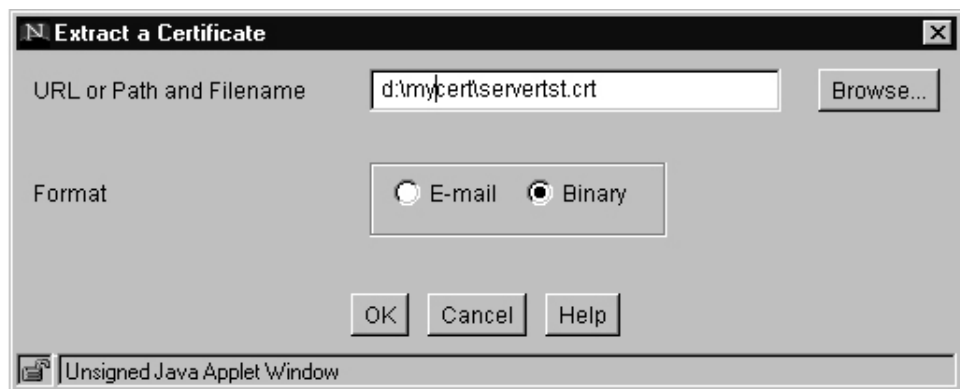
Figure 129. Extract a Certificate
