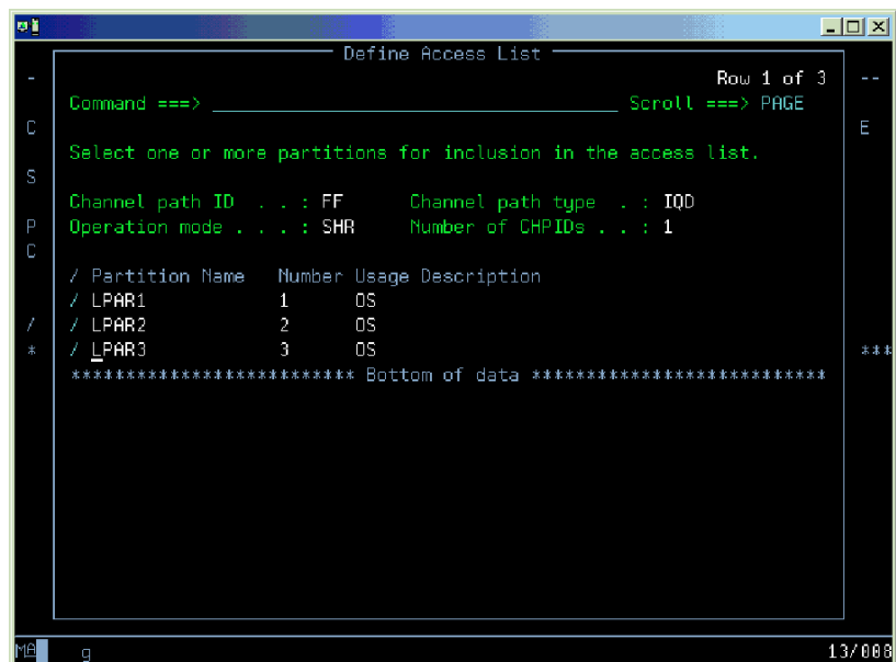
Figure 141. Define the channel path access list
