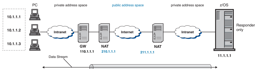
Figure 94. z/OS in a host-to-security gateway configuration
