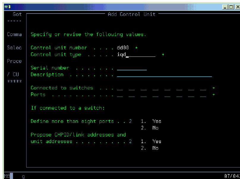
Figure 145. Define a control unit
