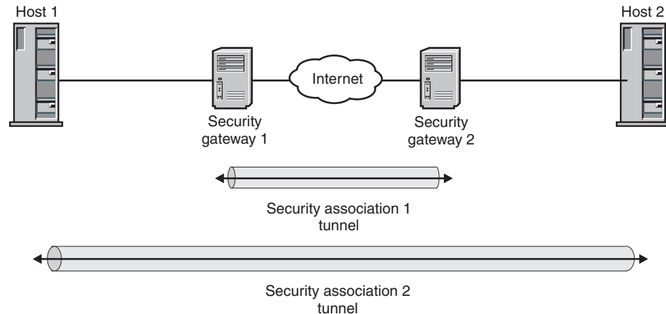
Figure 91. Nested tunnels
