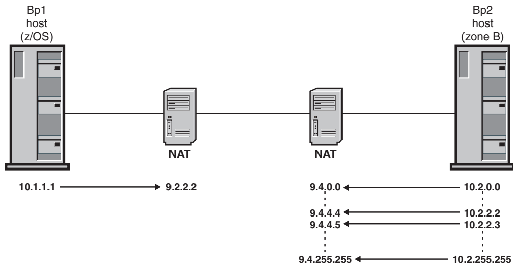
Figure 87. Business partner with NAT model
